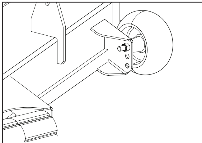
Anti-scalp rollers
